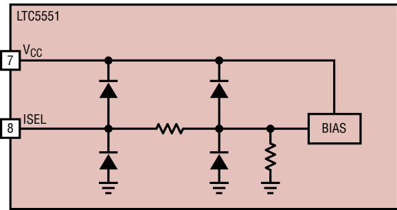
Figure 15. ISEL Interface Schematic
