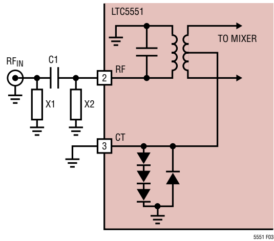
Figure 3. RF Input Schematic
