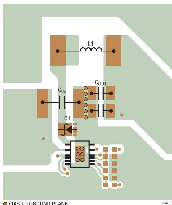
Figure 12. Example PCB Layout
