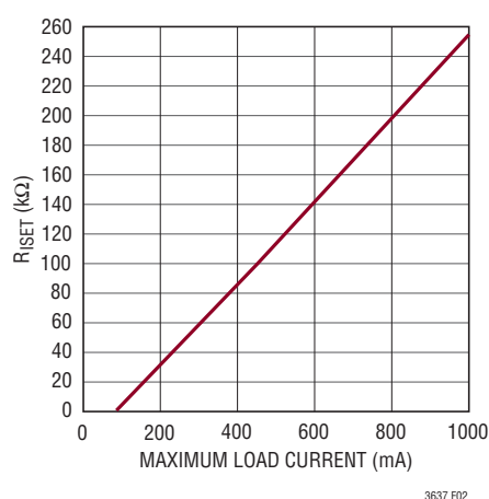
Figure 2. R_{ISET} Selection
