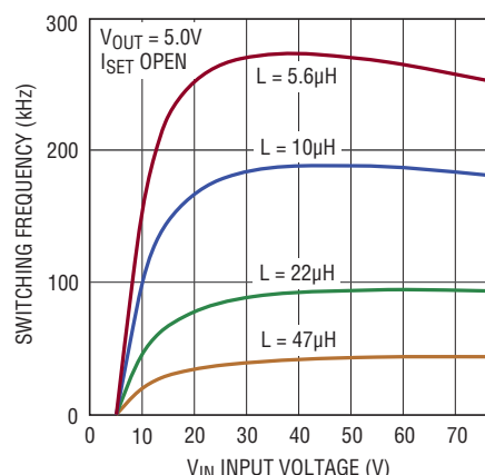
Figure 3. Switching Frequency for V_{OUT} = 5.0V
