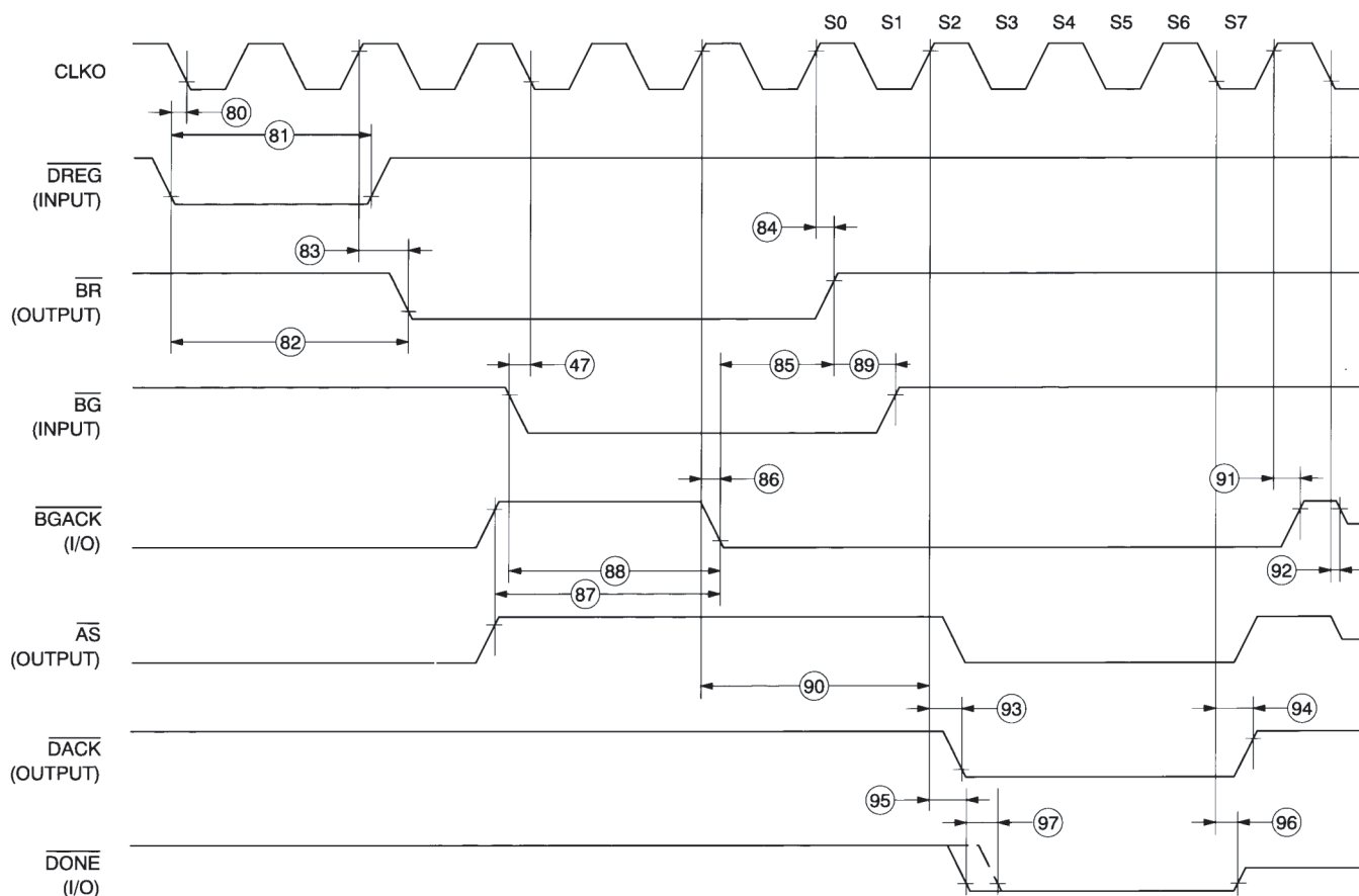
Figure 10. DMA Timing Diagram
